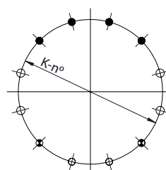
DN 10" - 14"
