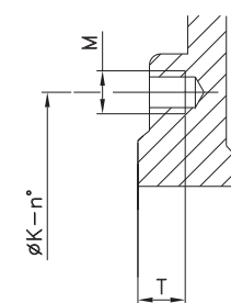
DN 450
