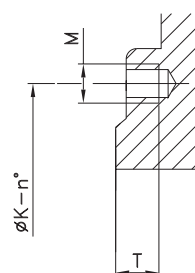
DN 10" - 14"
